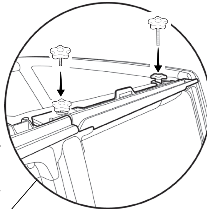
M8 x 75mm Knob #478.90 Qty. 2
